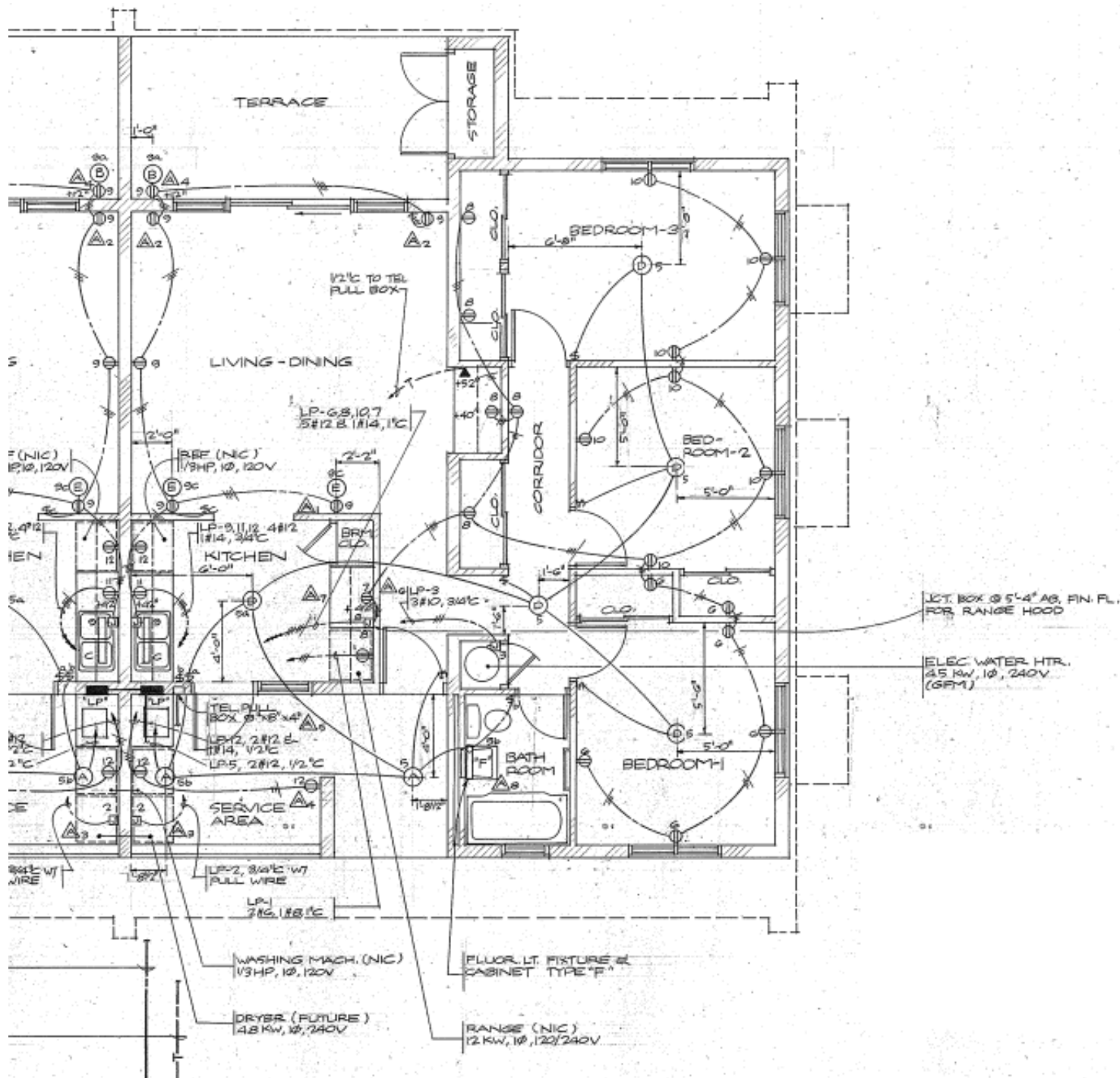
3BEDROOM FLOOR PLAN ELECTRICAL AS-BUILT
