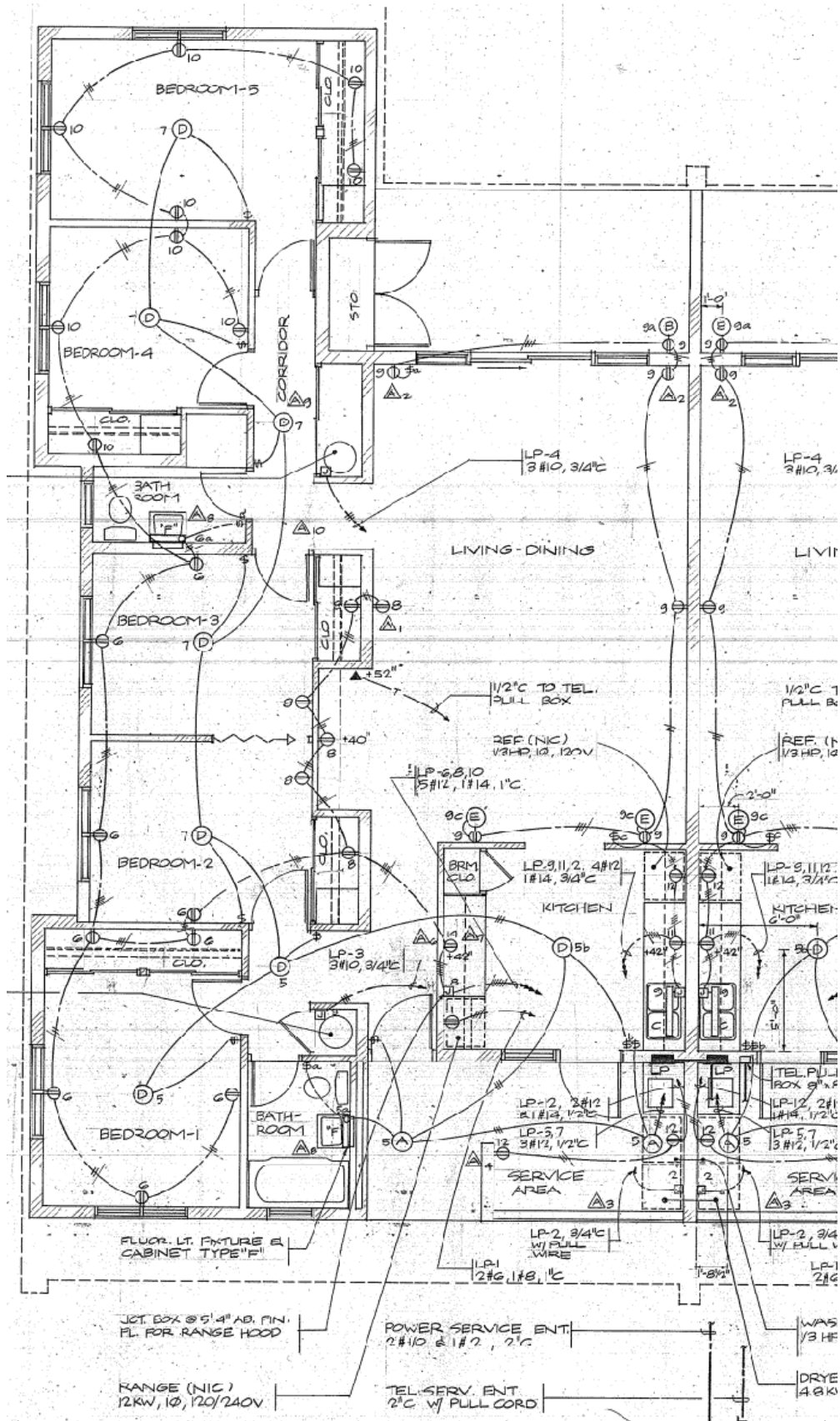
5 BEDROOM ELECTRICAL FLOOR PLAN AS-BUILT
