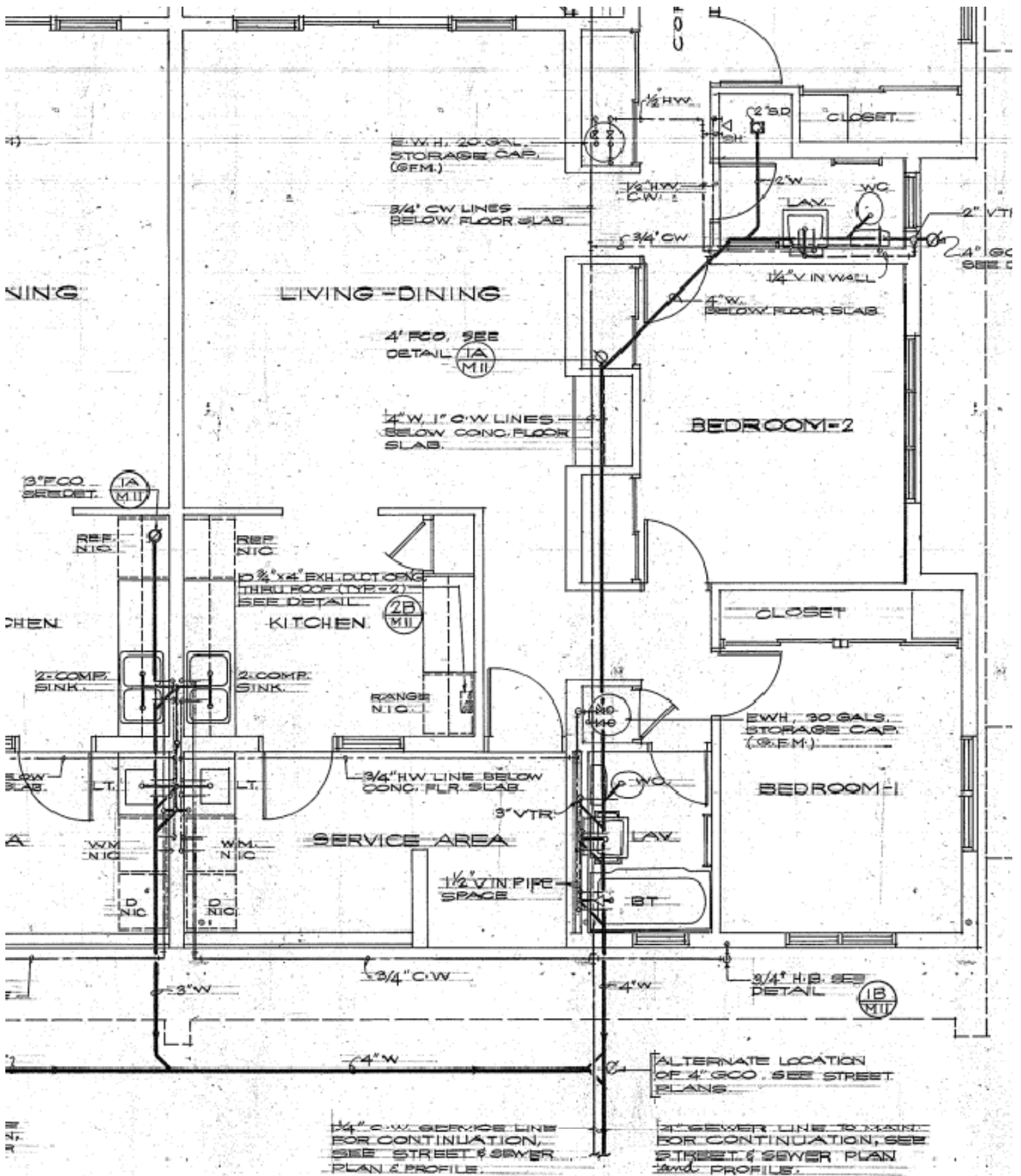
5 BEDRM. PLUMBING PLAN GH-250, AS-BUILT
