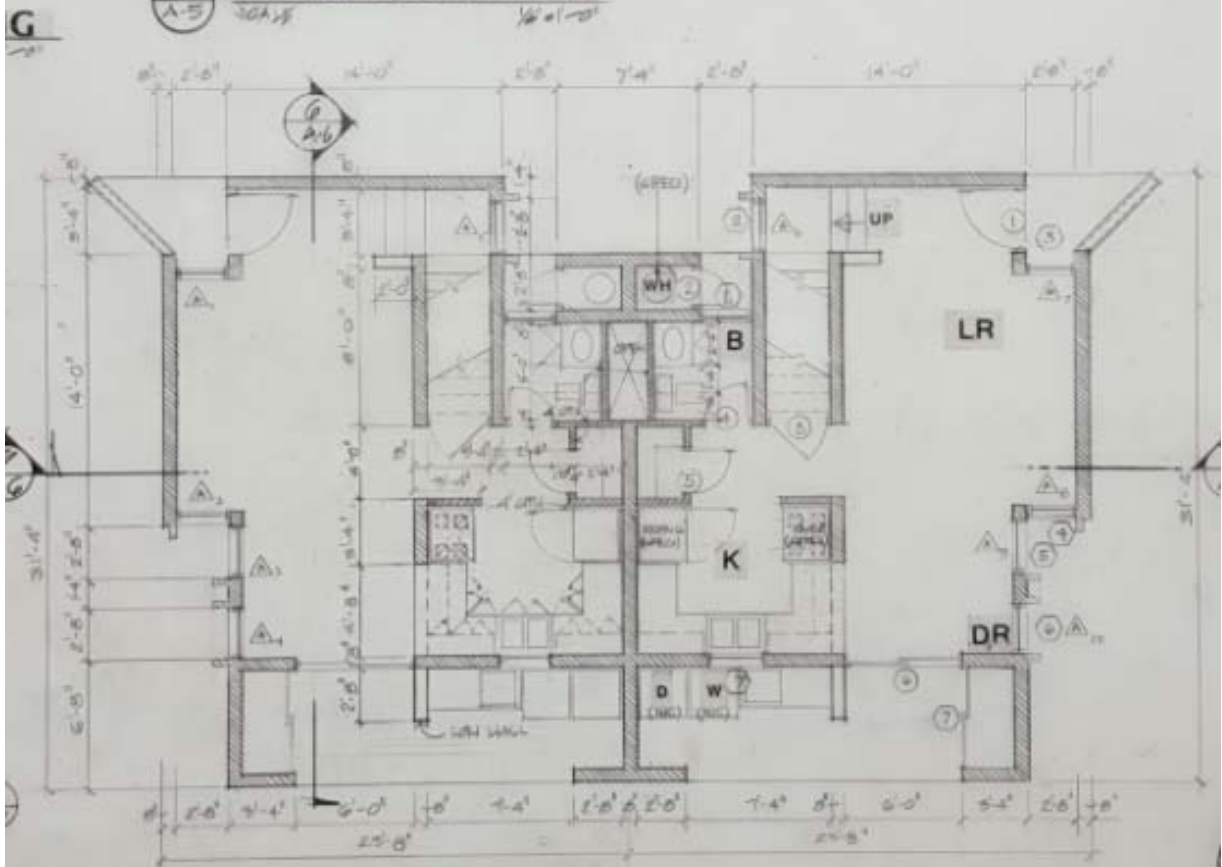
4 FIRST FLOOR PLAN 30A/2 1/8" = 1'-0"
