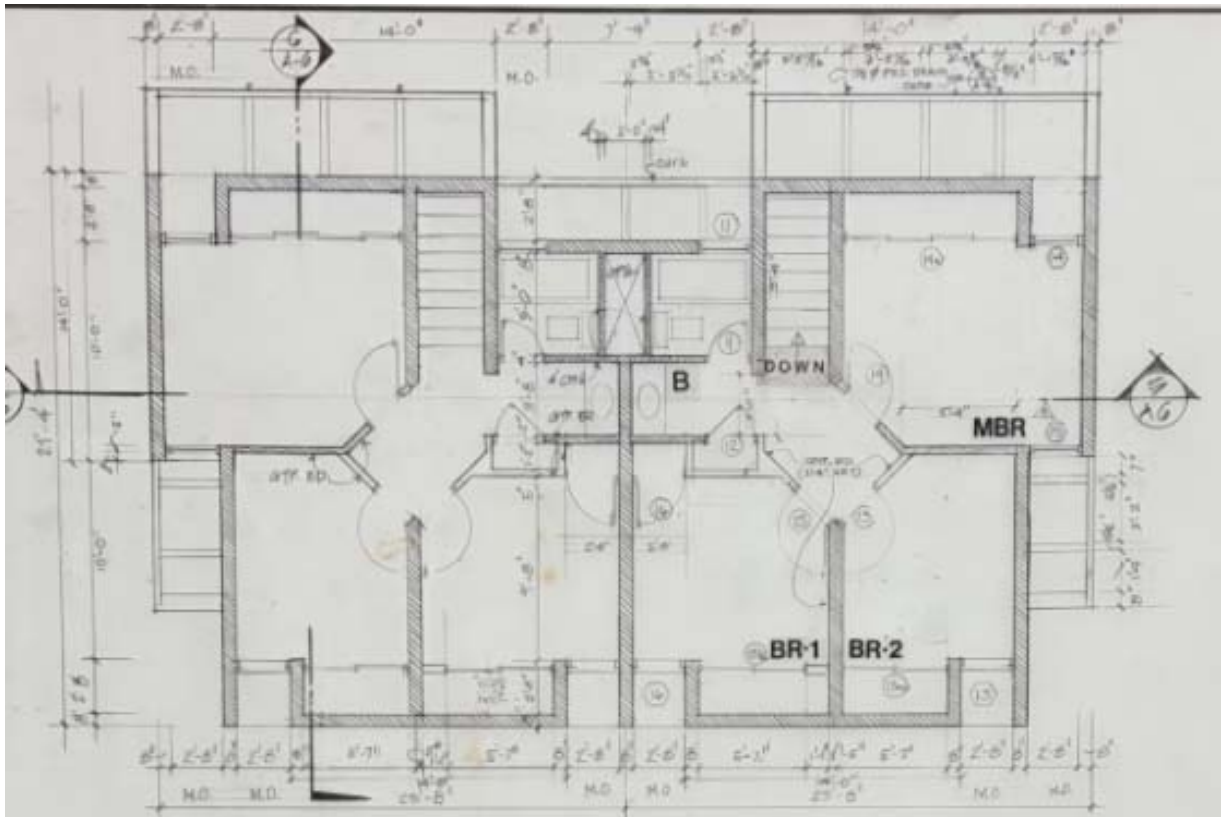
2 SECOND FLOOR PLAN 30A/2 1/8" = 1'-0"
