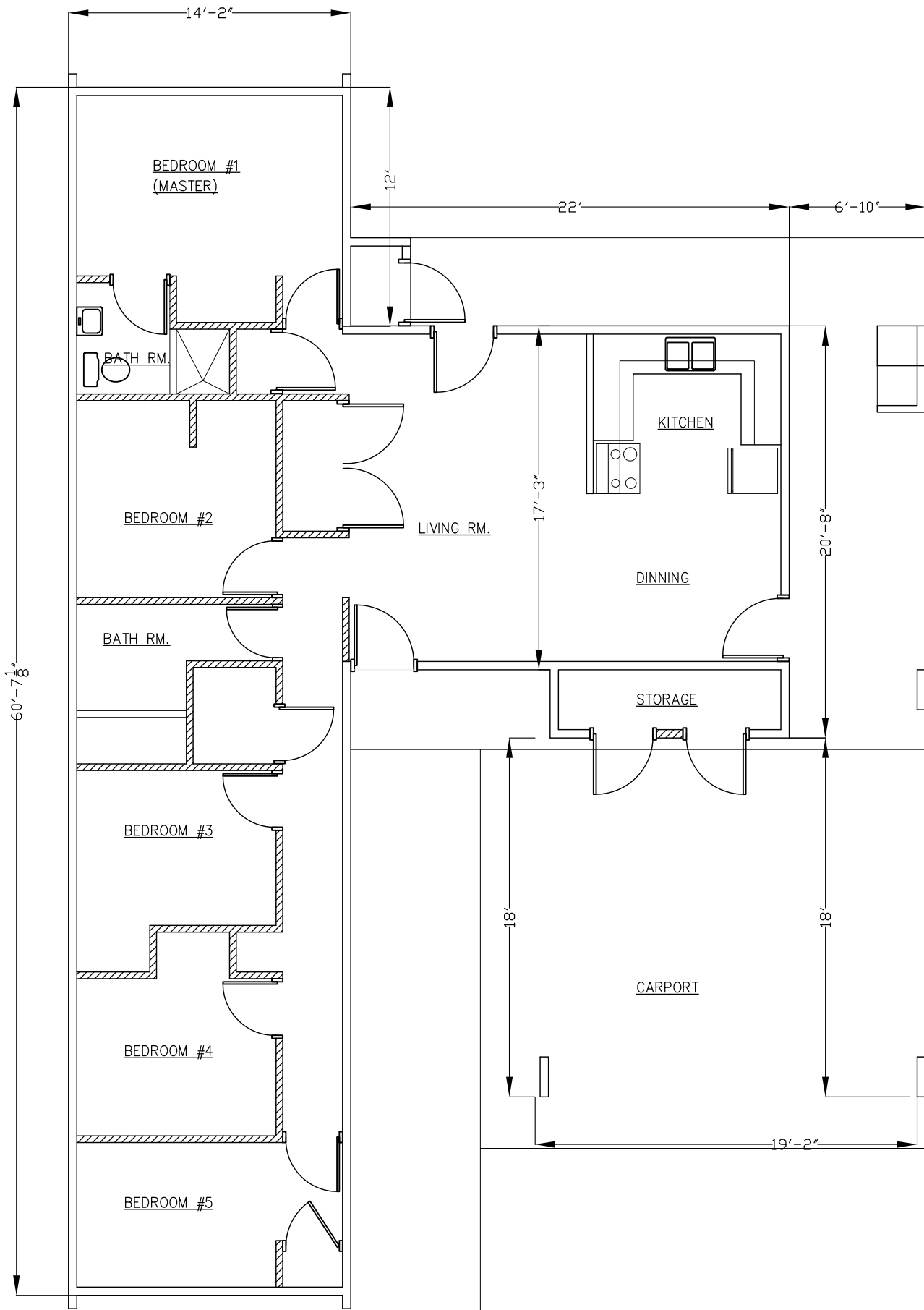
GH-99, 5-BEDROOM
