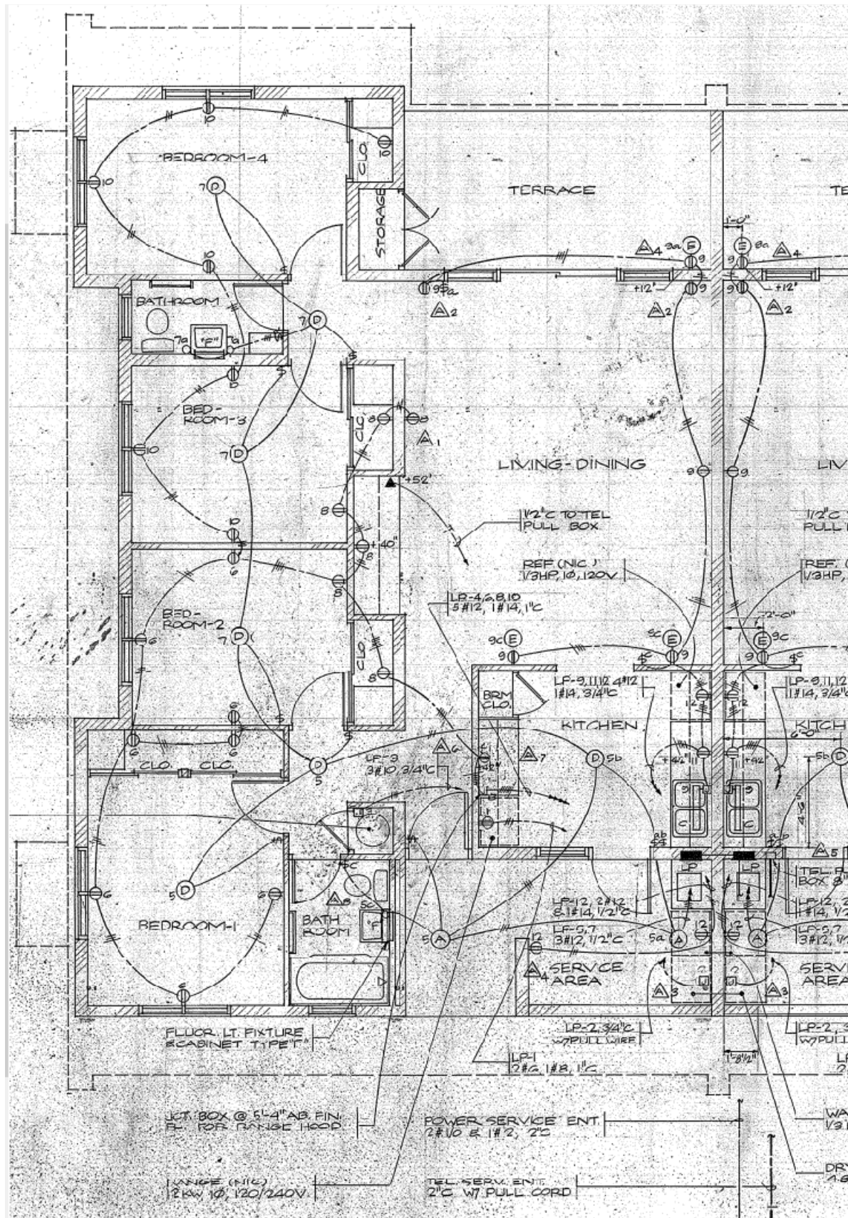
4 BEDROOM ELECTRICAL FLOOR PLAN AS-BUILT
