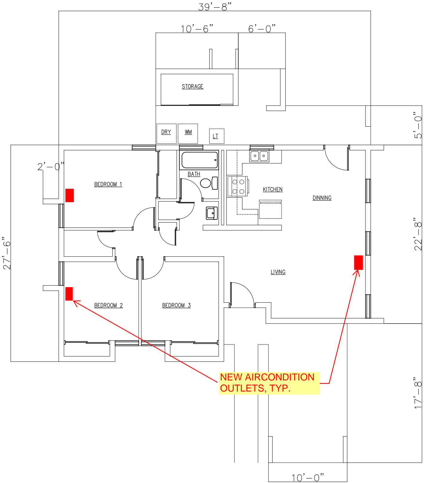
GH-35, 3-BEDROOM FLOOR PLAN
