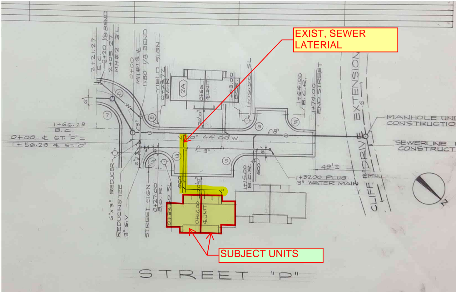
SITE UTILITY PLAN
