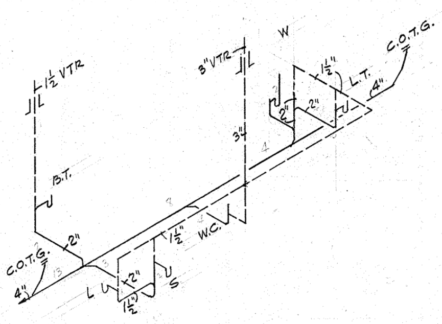
4 SANITARY PIPING DIAGRAM M-2 NO SCALE
