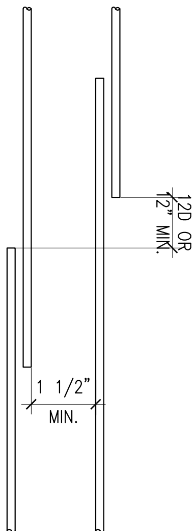
WALL/SLAB SPLICE DETAIL
